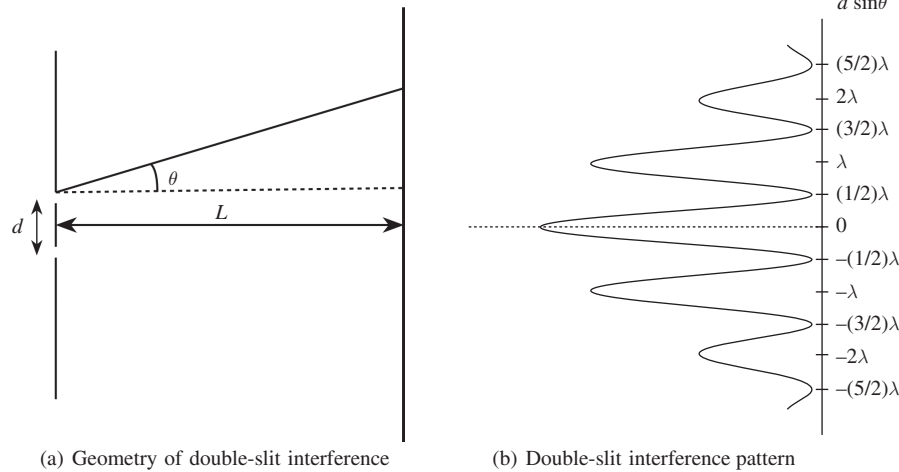
Figure 3.3 The interference pattern produced behind a double slit has a maximum when d \sin \theta is an integer multiple of the wavelength \lambda and a minimum when d \sin \theta is a half-integer multiple of the wavelength.
