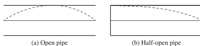
Figure 3.11 Snapshot at a single point in time of a pressure standing wave in a pipe with two ends open (a) or one end open (b). The point at the open end always must have a fixed pressure because it is open to the outside, which has constant pressure. Note that, confusingly, some references will draw similar figures to represent a snapshot of particle displacement in the wave. In that case, closed ends look like nodes, because the end of the pipe is fixed, and open ends look like antinodes. In either case, however, the wavelengths of the fundamental and its harmonics are the same.
