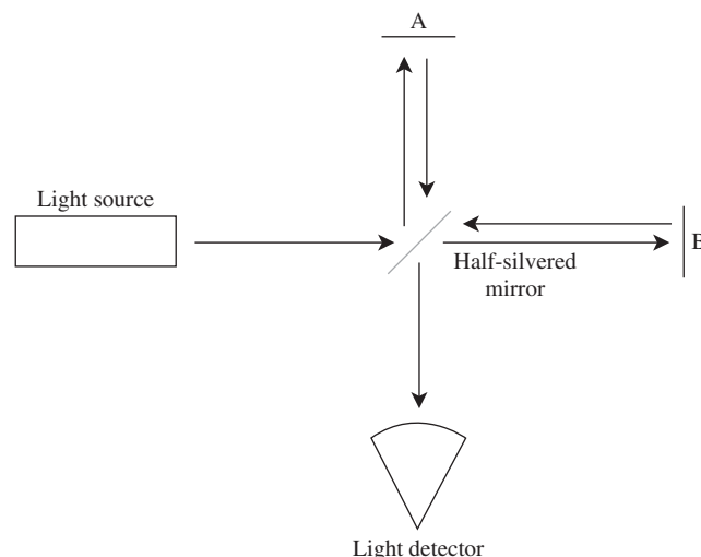
Figure 7.8 Michelson–Morley interferometer.
